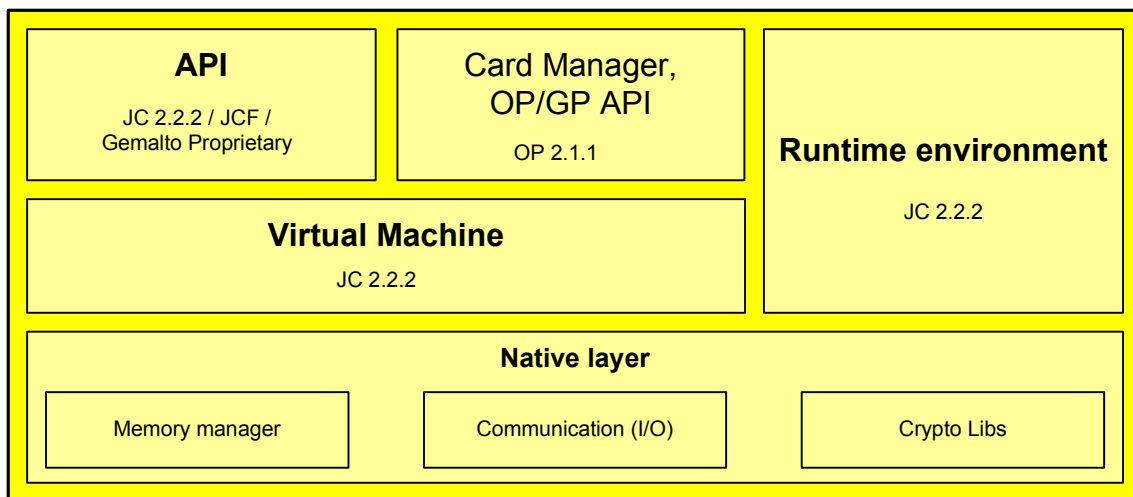
Figure 3: MultiApp ID V2.1 javacard platform architecture
