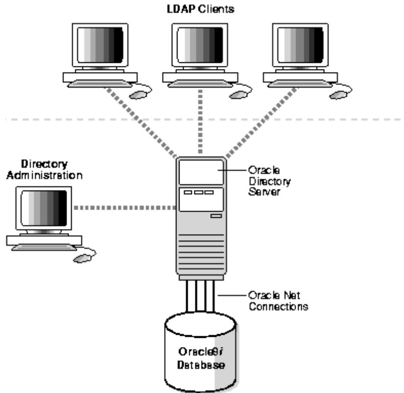
Figure 1: Oracle Internet Directory Architecture
