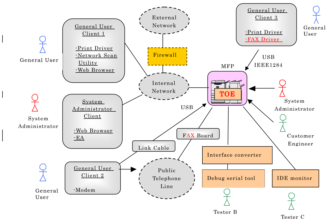
Figure 3-1 Configuration of Developer Testing
