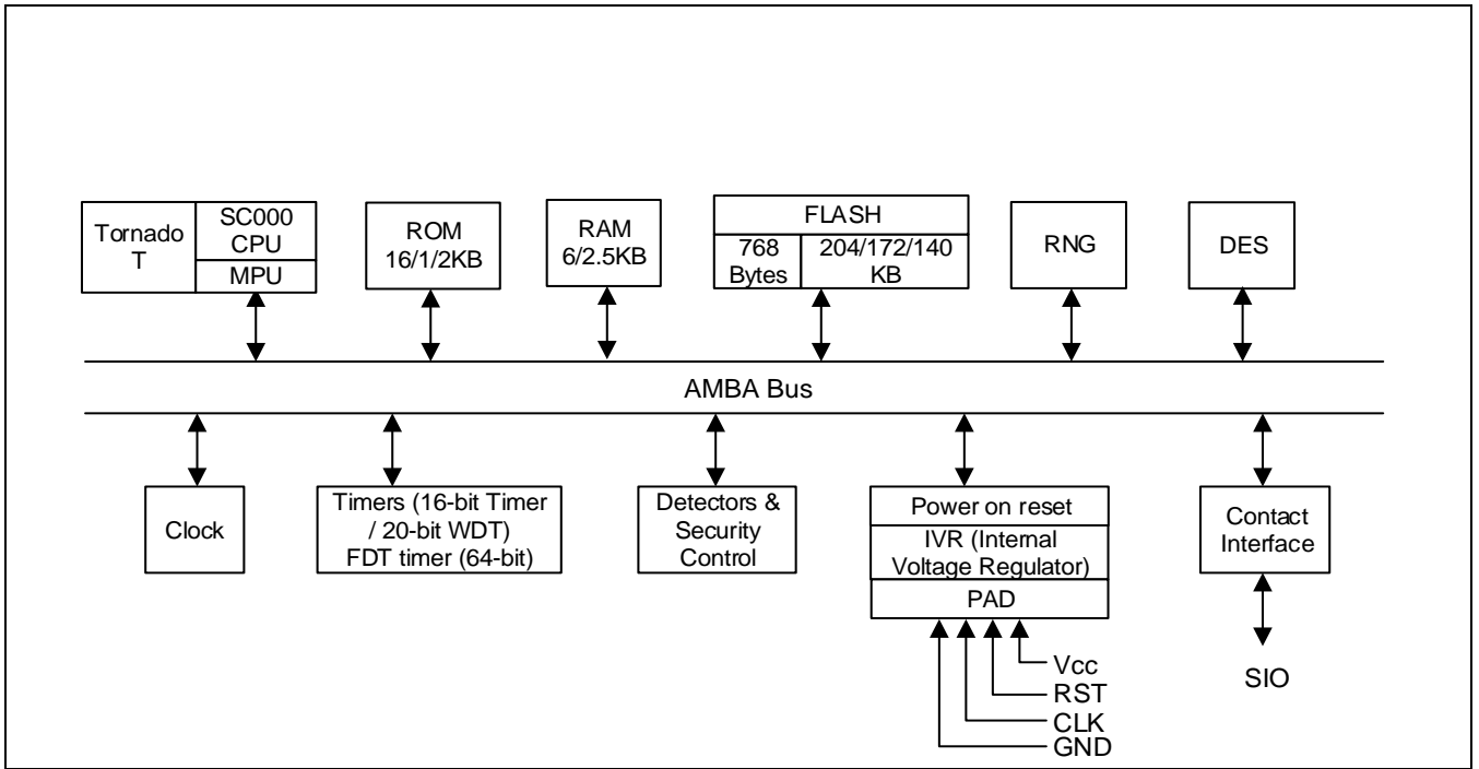
Figure 1 S3K200B/S3K170B/S3K140B Block Diagram
