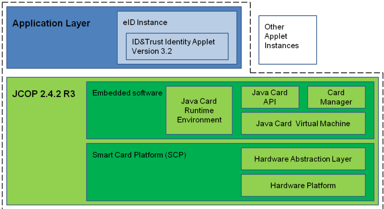
Figure 1 – The logical architecture of the TOE
