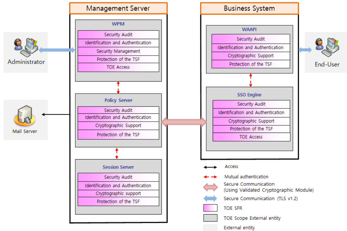
[Figure 2] TOE Logical scope
