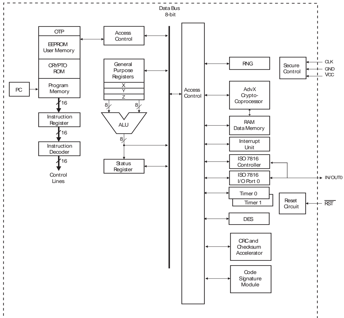
Figure 2-1 AT90SC20818RCU Block Diagram
