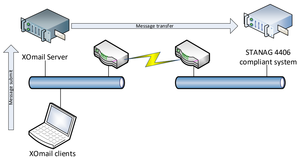
Figure 1-9 STANAG 4406 messaging
