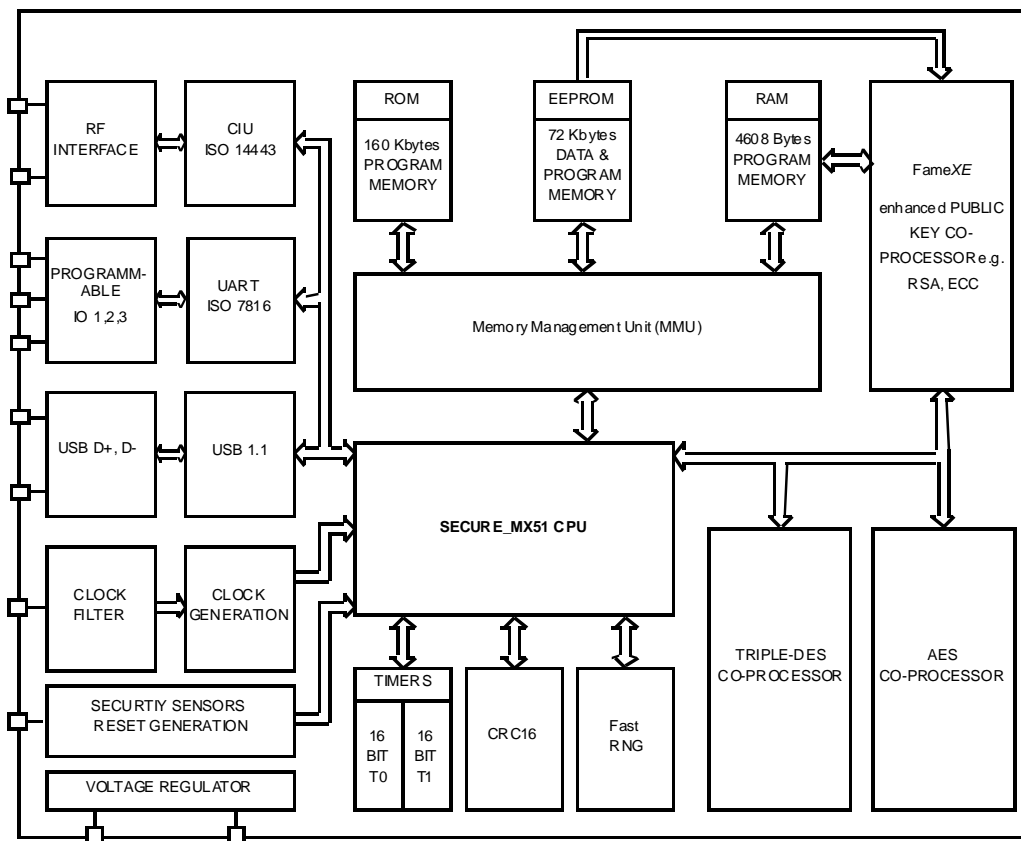
Figure 1: Block Diagram of the P5CT072V0Q
