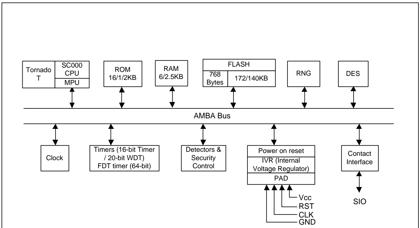
Figure 1 S3K170A/S3K140A Block Diagram
