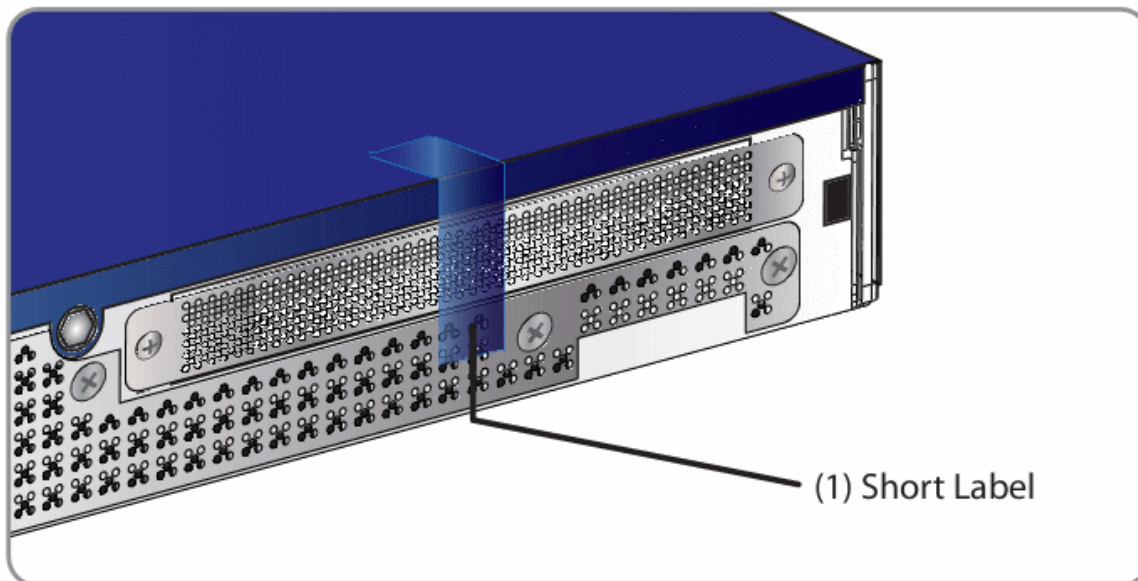
Figure 8 Tamper-Evident Label Placement over the PCI Cover
