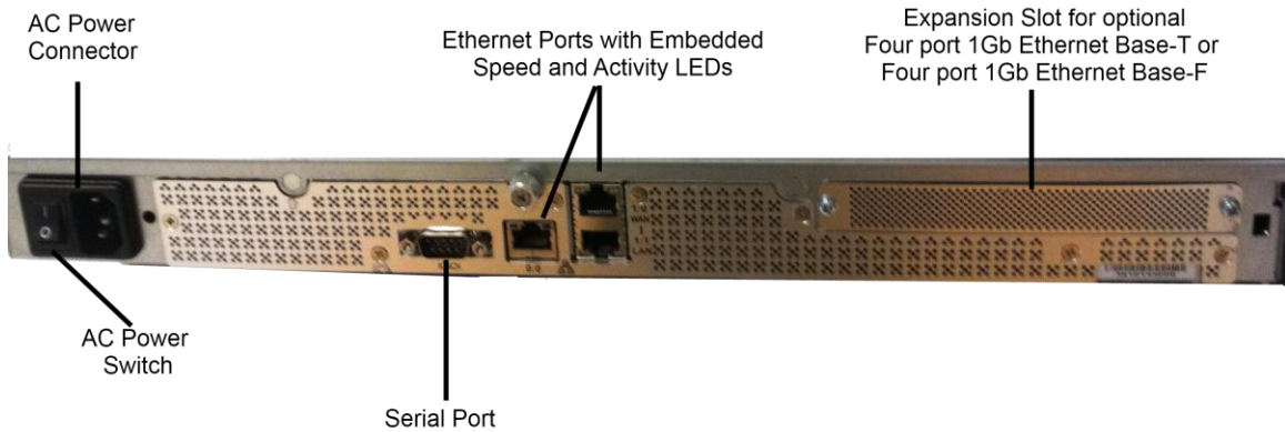
Figure 3 Connection Ports at the Rear of the SG600
