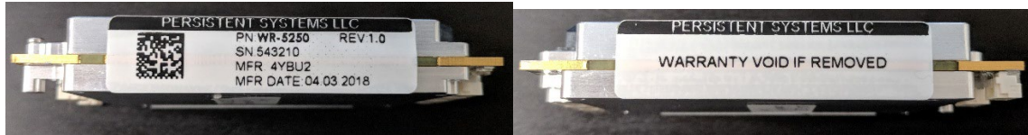
Figure 4 – Two Tamper-Evident Seals on sides of Embedded Module Lite
