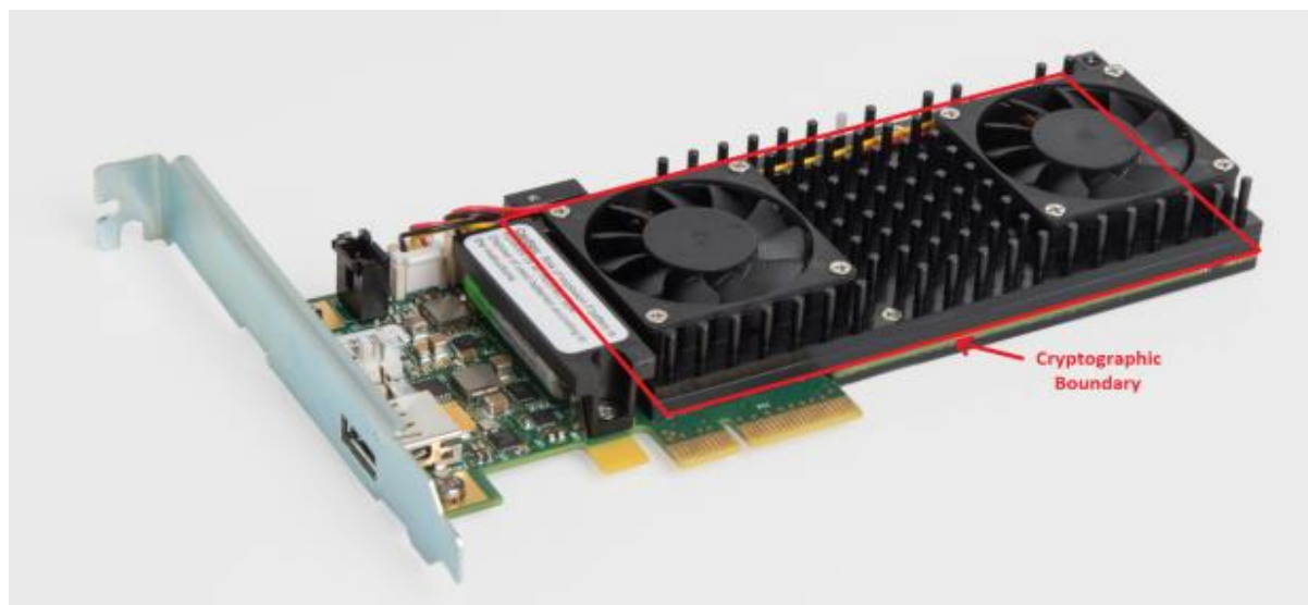
Figure 1: Thales Cryptovisor K7 Cryptographic Module cryptographic boundary
