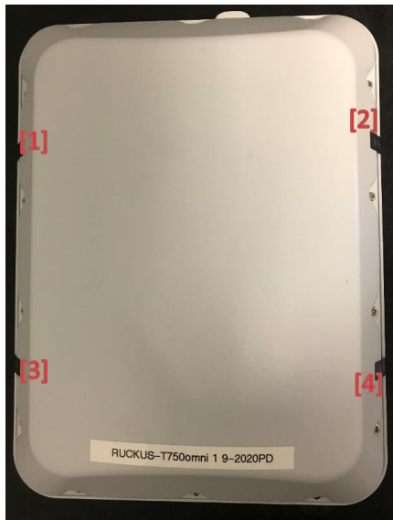
Figure 34: T750/T750-WW Top
