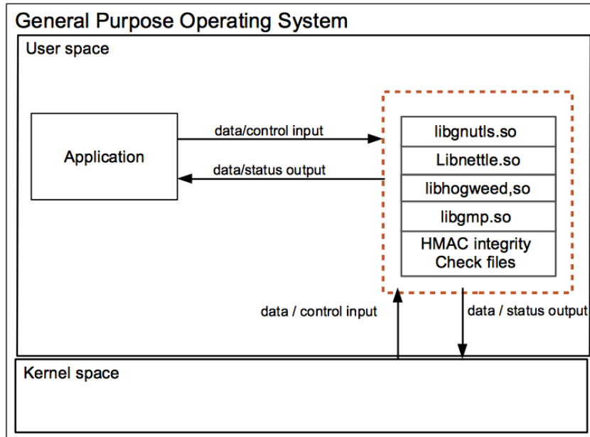
Figure 1: Oracle Linux 7 GnuTLS Logical Cryptographic Boundary
