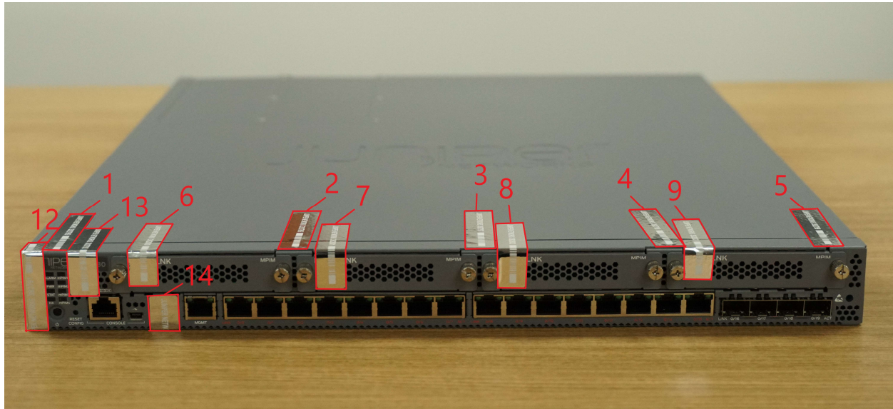
Figure 10 – SRX 380 Tamper-Evident Seal Placement (Rear)
