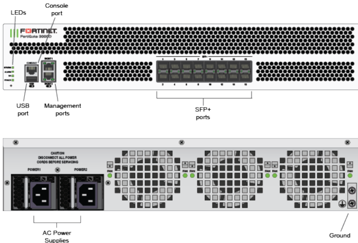
Figure 8 - FortiGate-3000D Front and Rear Panels
