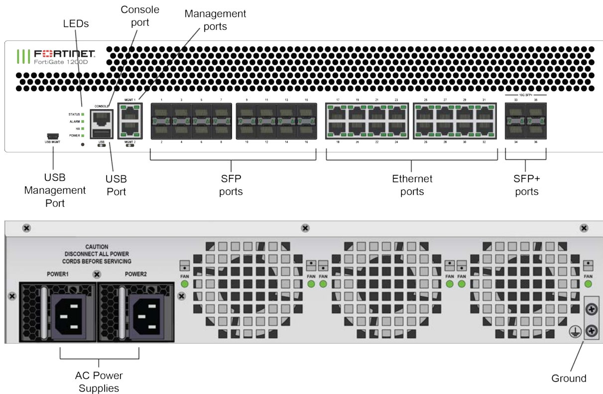
Figure 6 - FortiGate-1200D Front and Rear Panels
