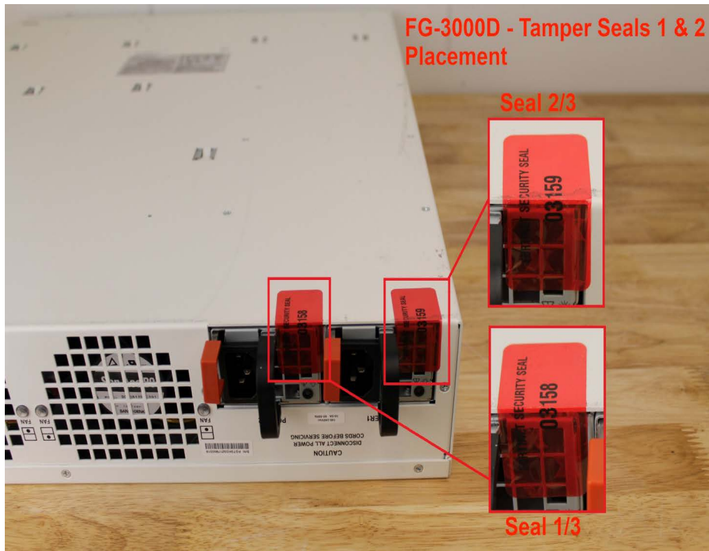
Figure 18 - FortiGate-3000D external enclosure seals, rear, bottom
