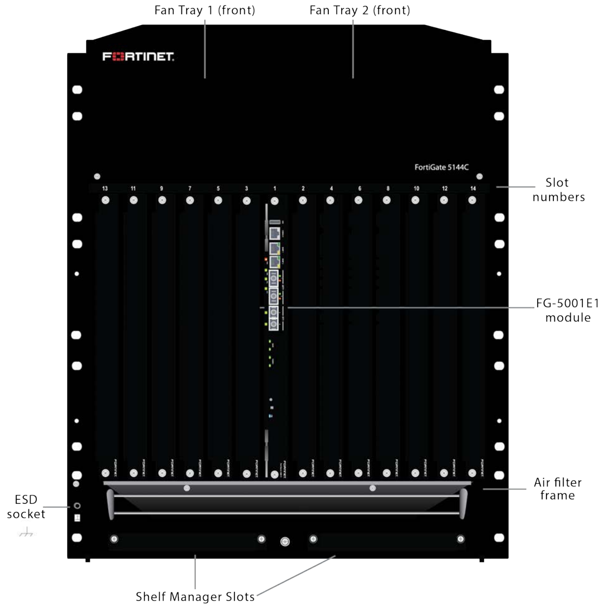
Figure 3 - FortiGate-5144C Front Panel
