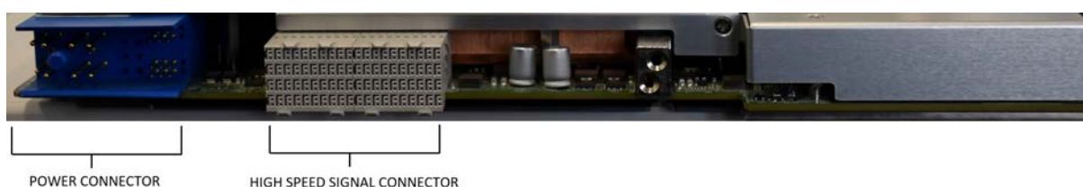
Figure 2 - FortiGate-5001D Rear Blade Connectors
