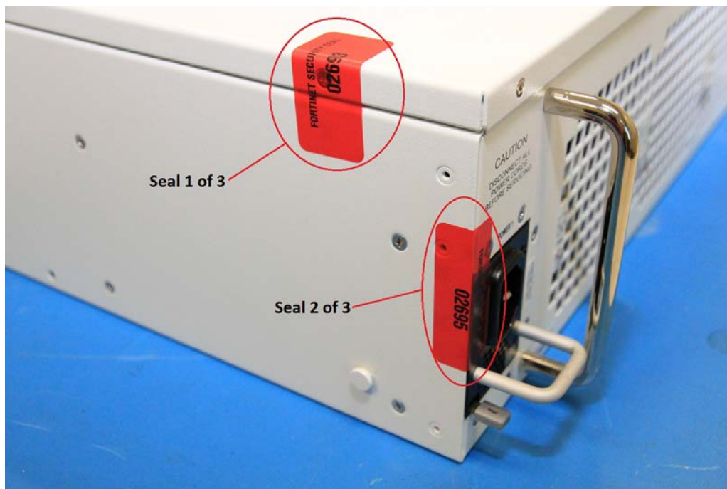
Figure 20 - FortiGate-3700D external enclosure seal and power supply seal, right, rear
