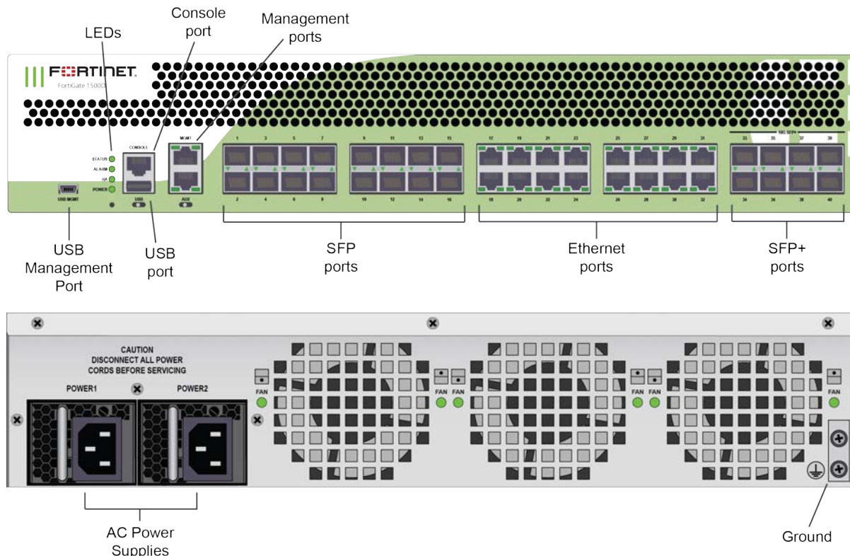
Figure 7 - FortiGate-1500D Front and Rear Panels
