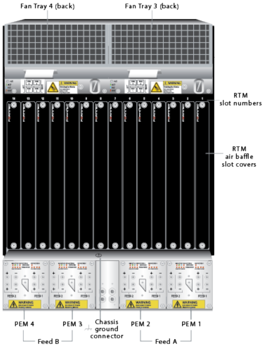
Figure 4 - FortiGate-5144C Rear Panel
