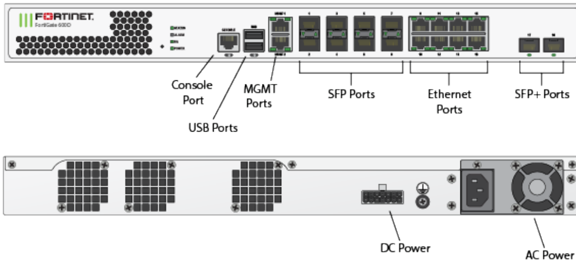
Figure 5 - FortiGate-600D Front and Rear Panels
