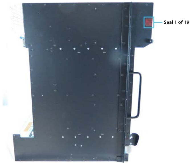
Figure 10 - FortiGate-5001D seals, left side view
