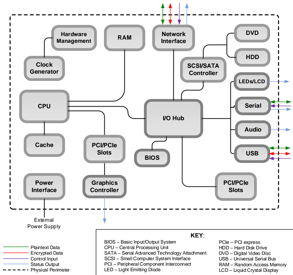
Figure 1 – GPC Block Diagram
