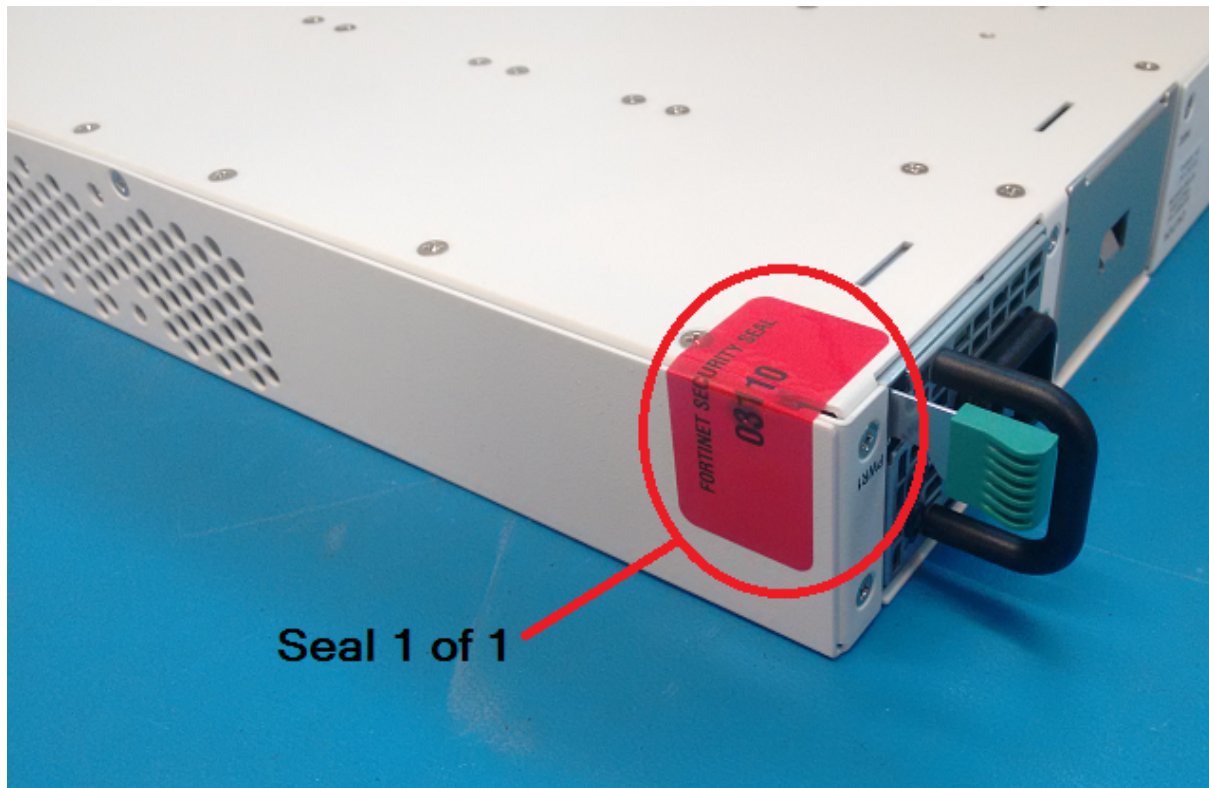
Figure 5 - FortiGate-301E, 401E, 501E and 601E external enclosure seal, bottom, rear side
