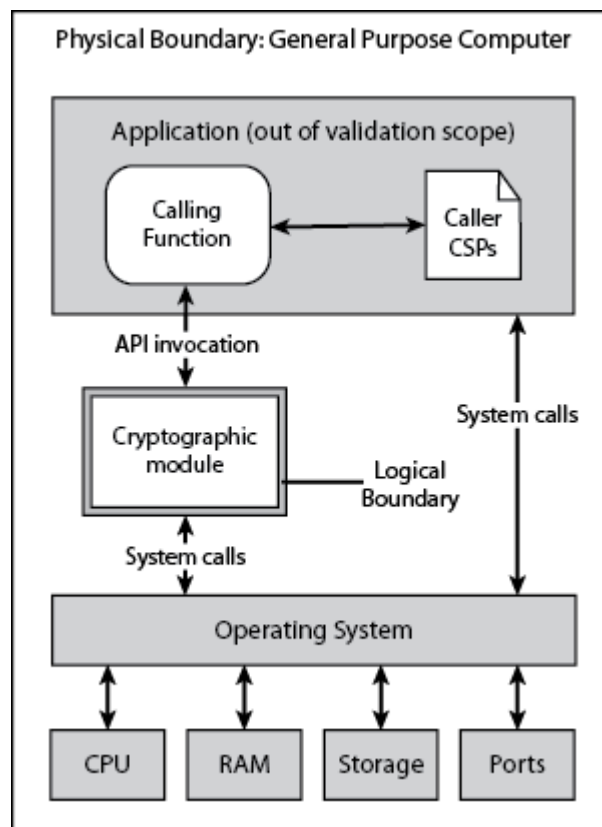
Figure 1 – Logical Boundary
