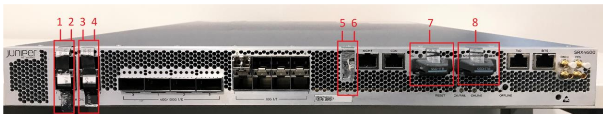
Figure 18 - SRX4600 Front View: TEL 1 – 8
